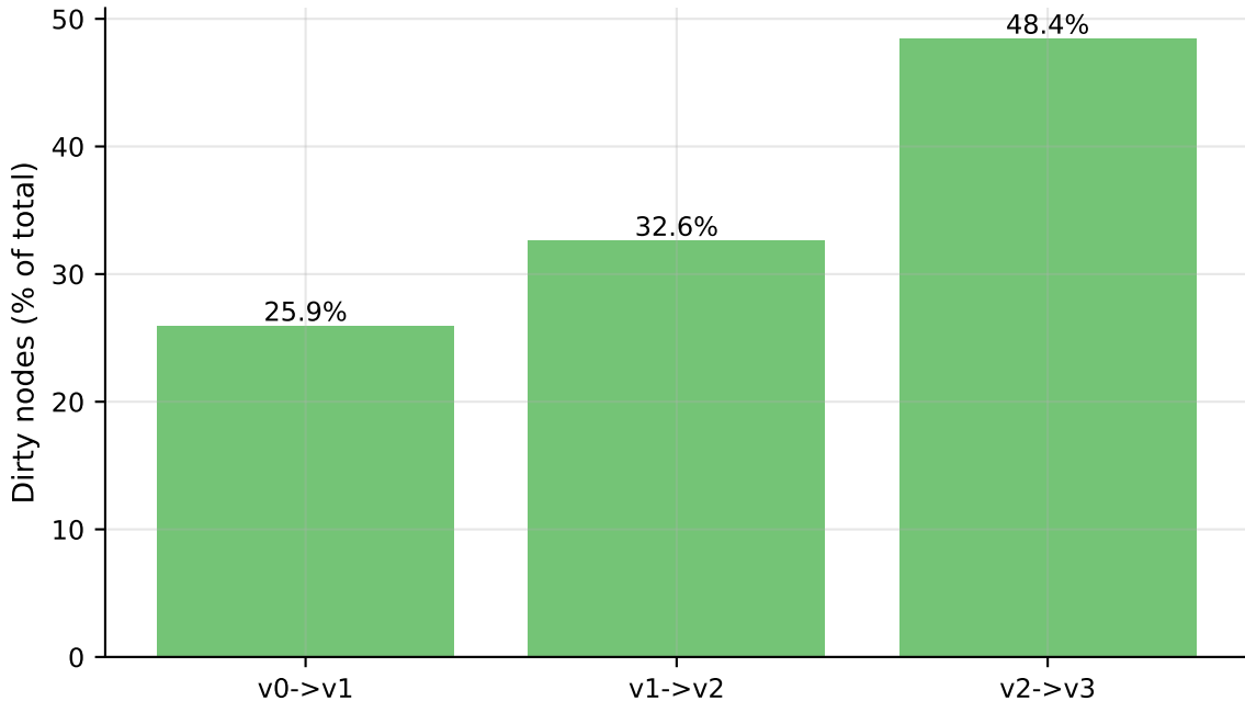
Group C - Localised update: dirty-set size as graph grows
